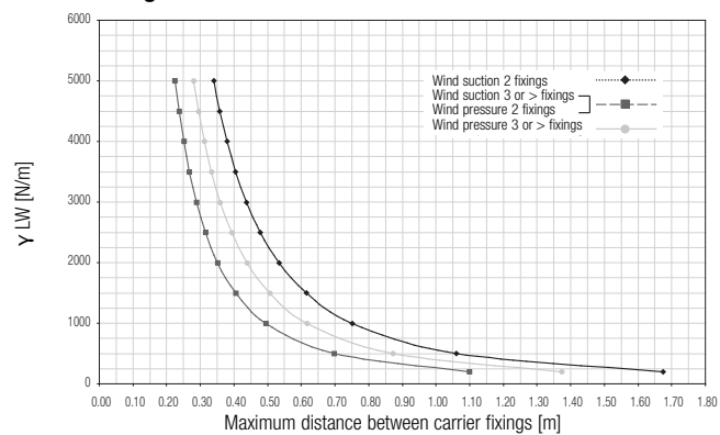
Design chart of carrier 84B
